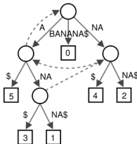
A suffix tree of "BANANA$" (from Wikipedia ).
