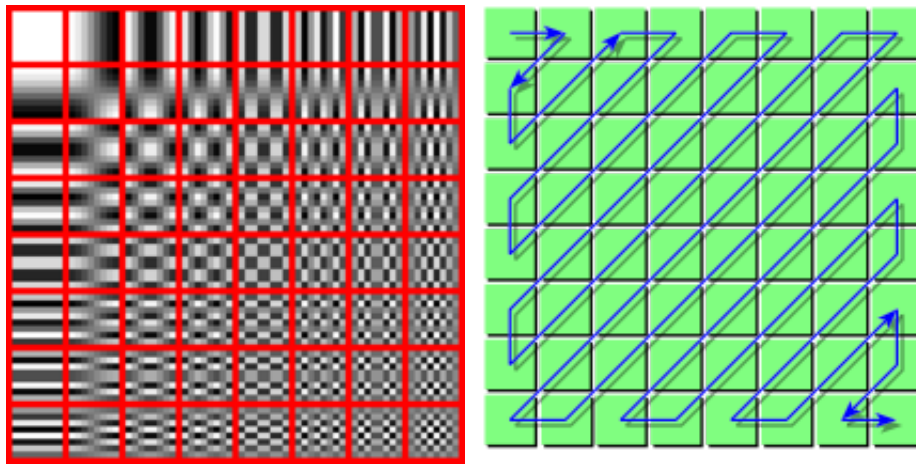
Left: 8 by 8 DCT (from Wikipedia ). Right: zig-zag encoding order of the S_{uv} coefficients (from Wikipedia ).
